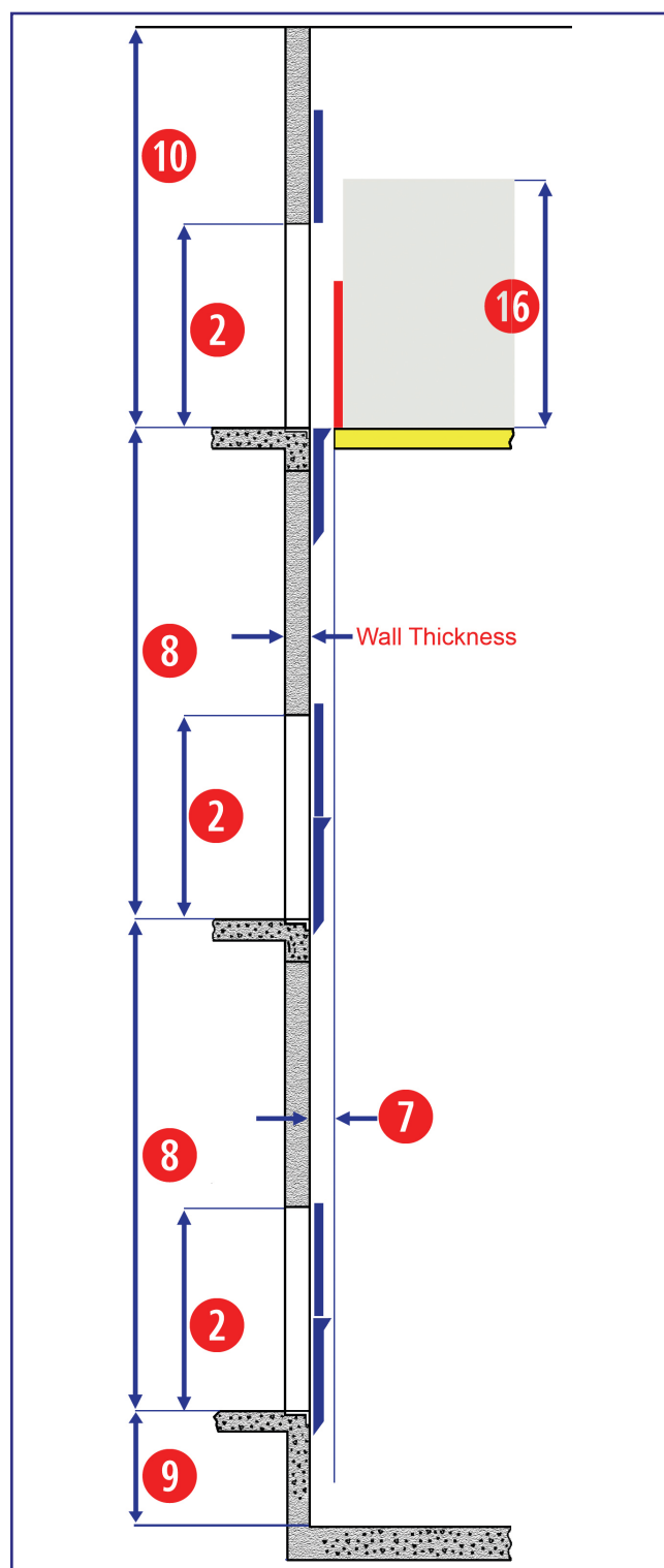
Hoistway Vertical View
