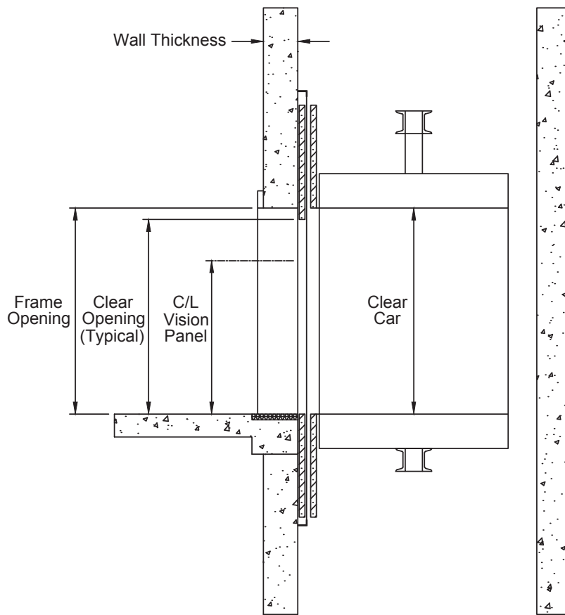
Elevation View
