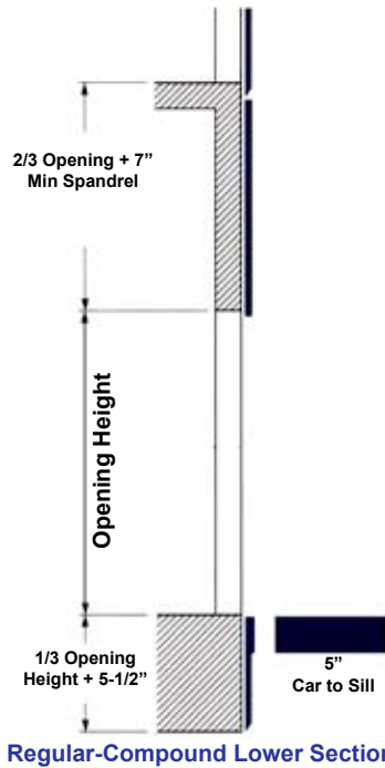
Regular-Compound Lower Section
