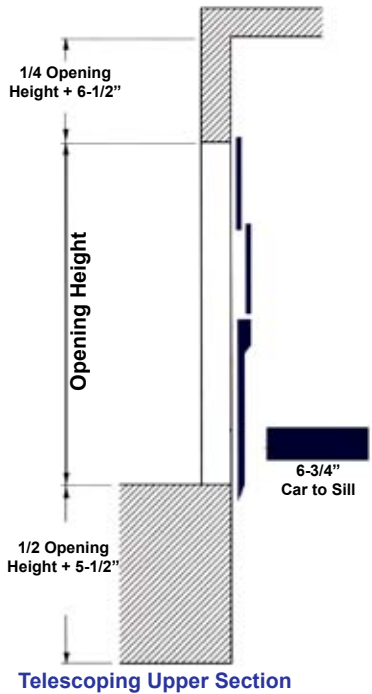
Telescoping Upper Section
