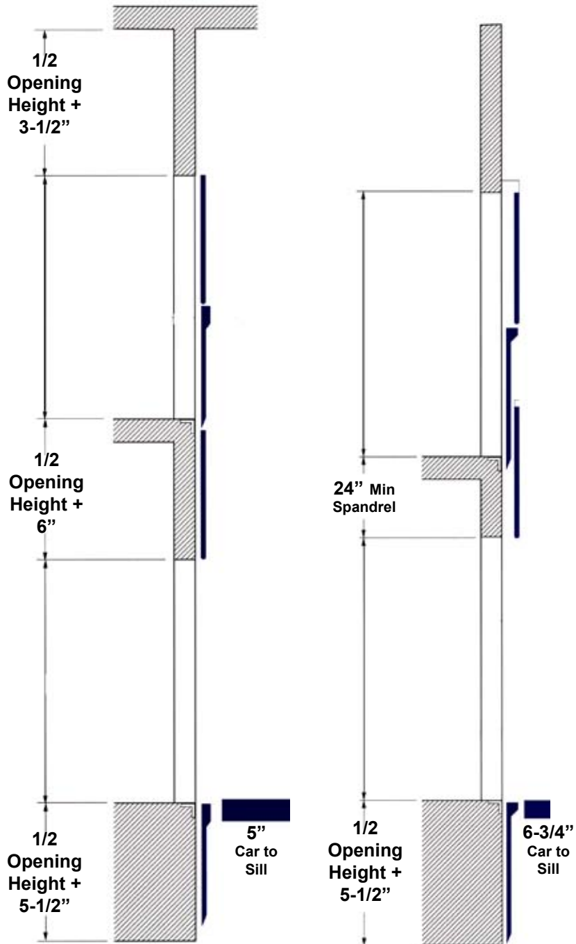
Regular Type Doors
