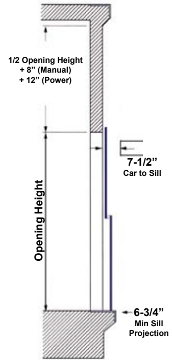
Two-Section Slide-Up
